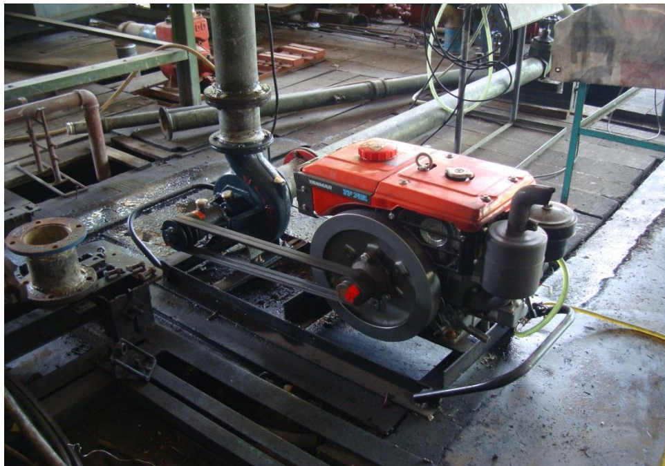
Figure 1. SAKAI 4 x 4 Centrifugal pump coupled to YANMAR TF70L Diesel engine on the test set-up
