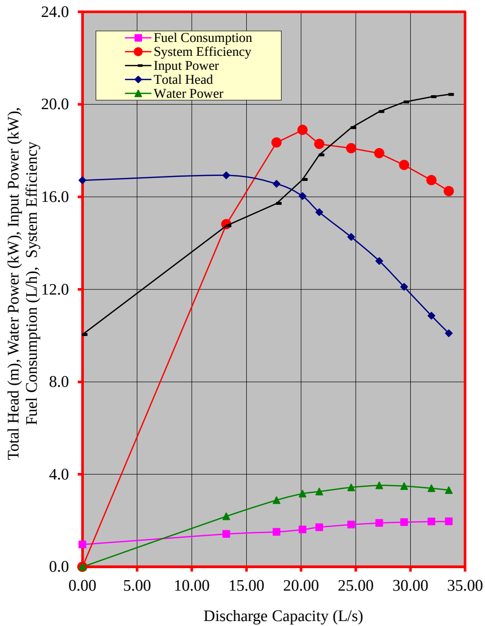
Figure 2. Performance characteristic curves of the SAKAI 4 x 4 centrifugal pump coupled to YANMAR TF70L diesel engine
